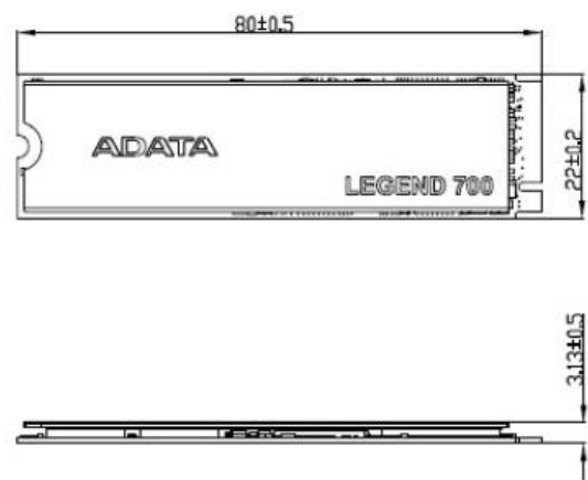
<With heatsink>
