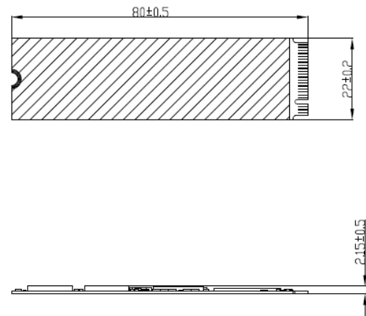
<Without heatsink>
